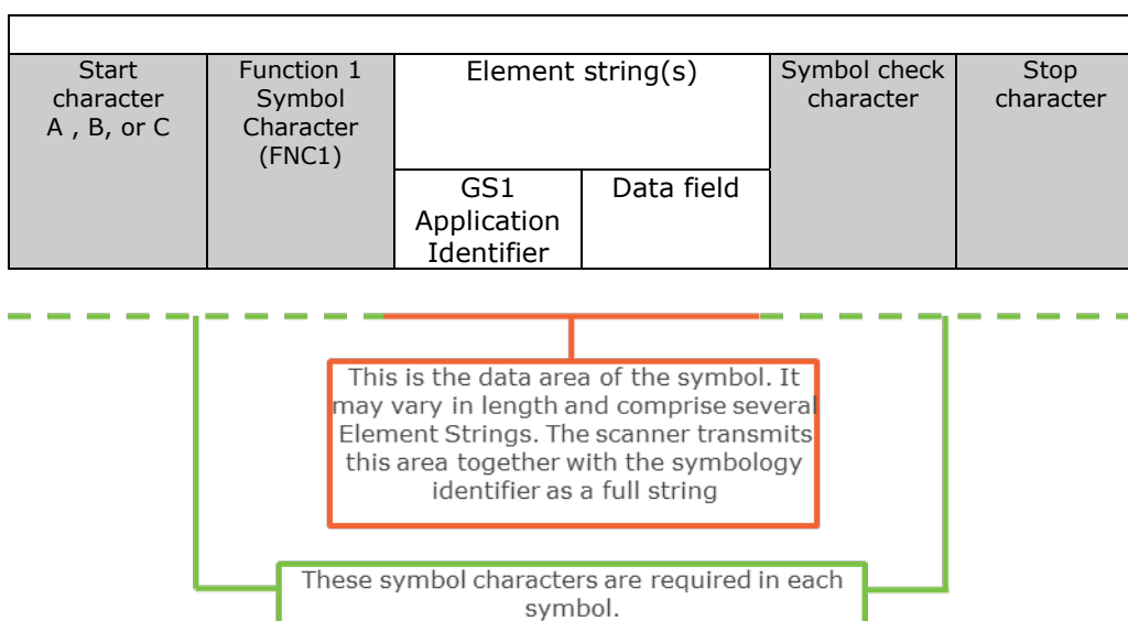
Figure 7.8.5-1. Example GS1-128 barcode structure
