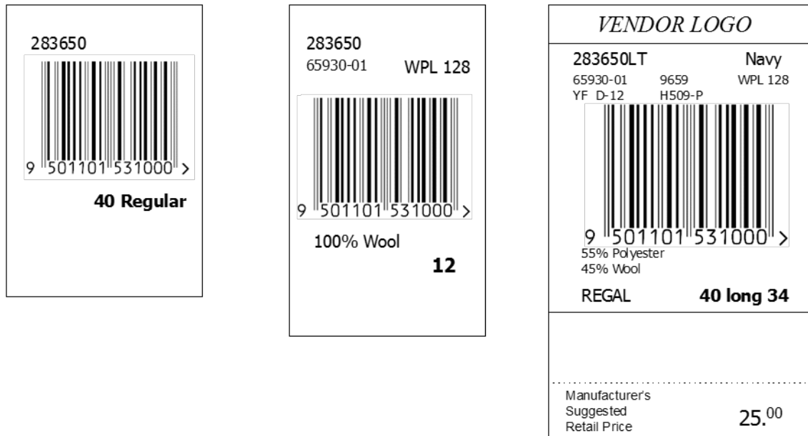
Figure 6.5.3.2-2. Horizontal layout
