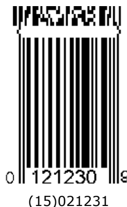
Figure 7.8.6.3-2. Example of mixed GS1 symbologies (GTIN encoded in UPC-E, Best before date in Composite)
